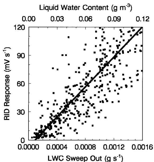
FIG. 15. Scatterplot of LWC sweep out vs RID for liquid phase cases with LWC <0.15 g m -3 and temperature <-5°C (485 points). The best fit has an LWC of 0.007 ± 0.010 g m -3 for an RID signal of 0 mV. The equivalent LWC is shown for comparison.
